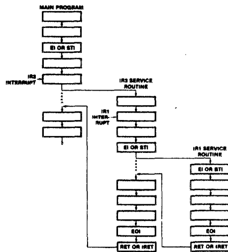
Figure 12. Fully Nested Mode Example (MCS 80/85™ or MCS 86/88™)
