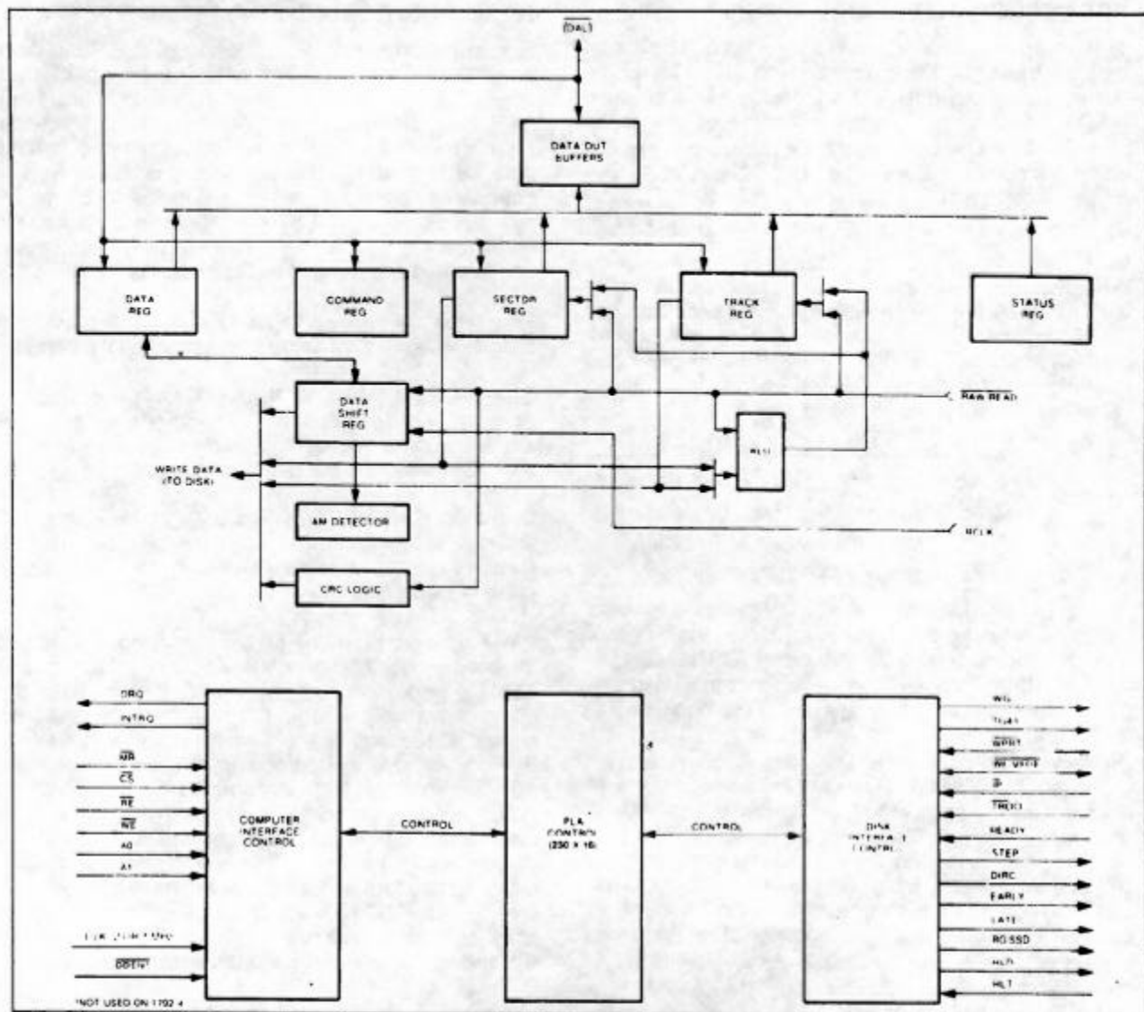
FD179X BLOCK DIAGRAM
