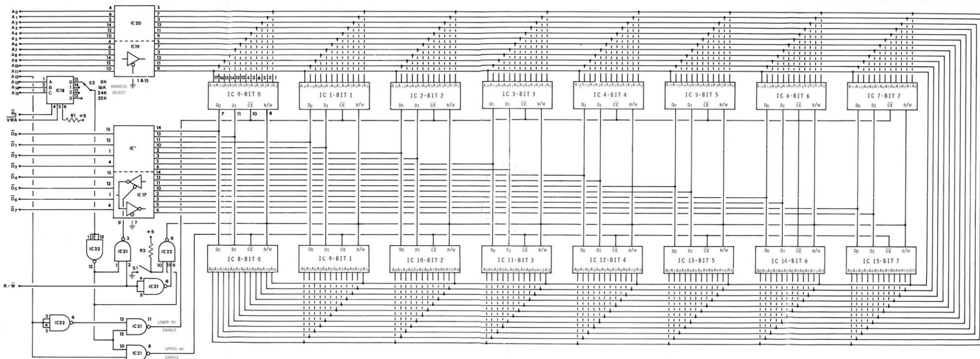
MP-8M2 Memory Board Schematic
