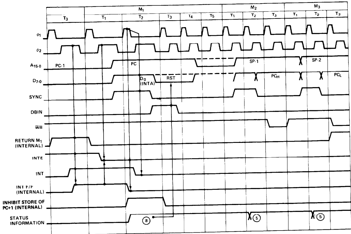
PICTORIAL 7-8 Interrupt Timing
