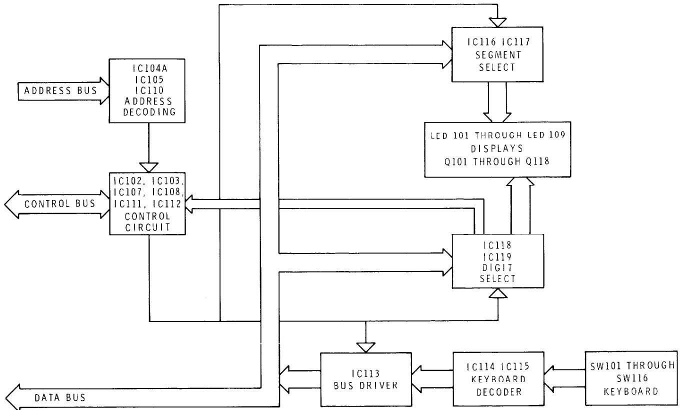
CONTROL BLOCK DIAGRAM
